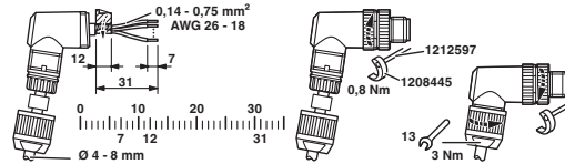
Functional drawing
